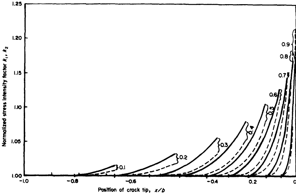
Fig. 6. Effect of the first reflected stress wave on the dynamic stress intensity factor for the different values of v/c shown. The dynamic stress intensity factors are given in the normalized forms of eqns (37) and (38) so that k_1 (full lines) and k_2 (dashed lines) give the contributions from the u^{-1/2} and u^{+1/2} terms for the stress ahead of the original crack tip respectively.
